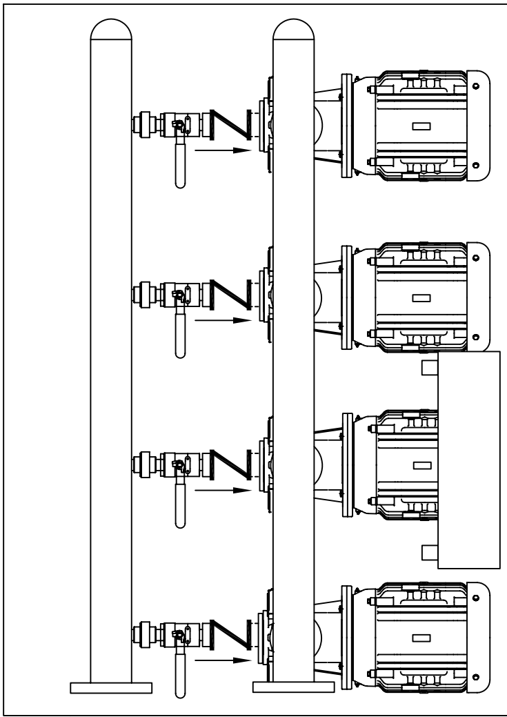
TOP-VIEW
