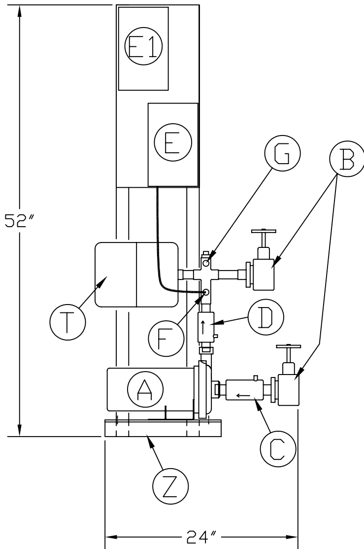
SIDE - VIEW
